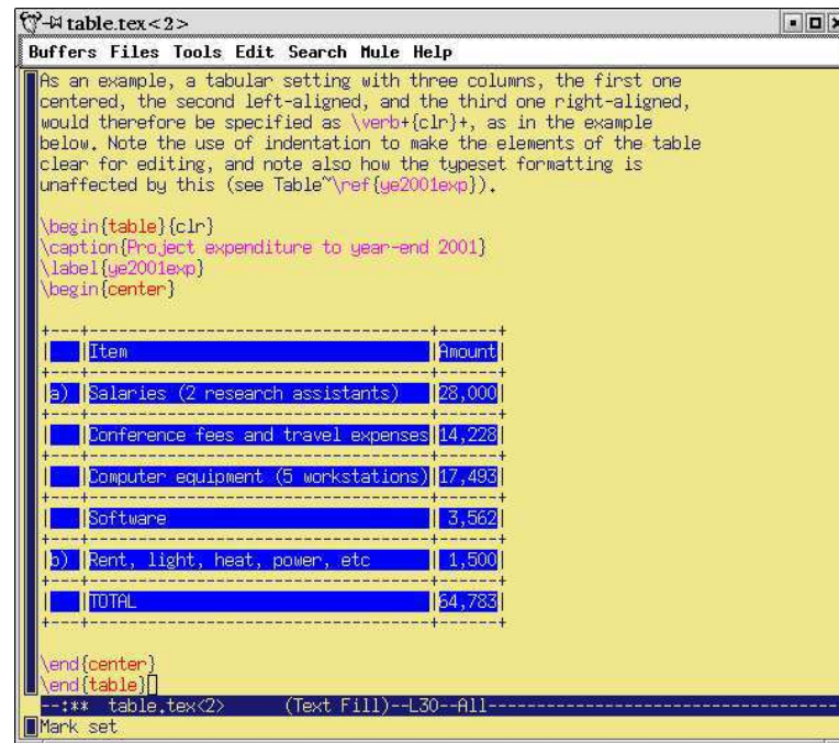
Figure 6.1: Tables mode for Emacs
